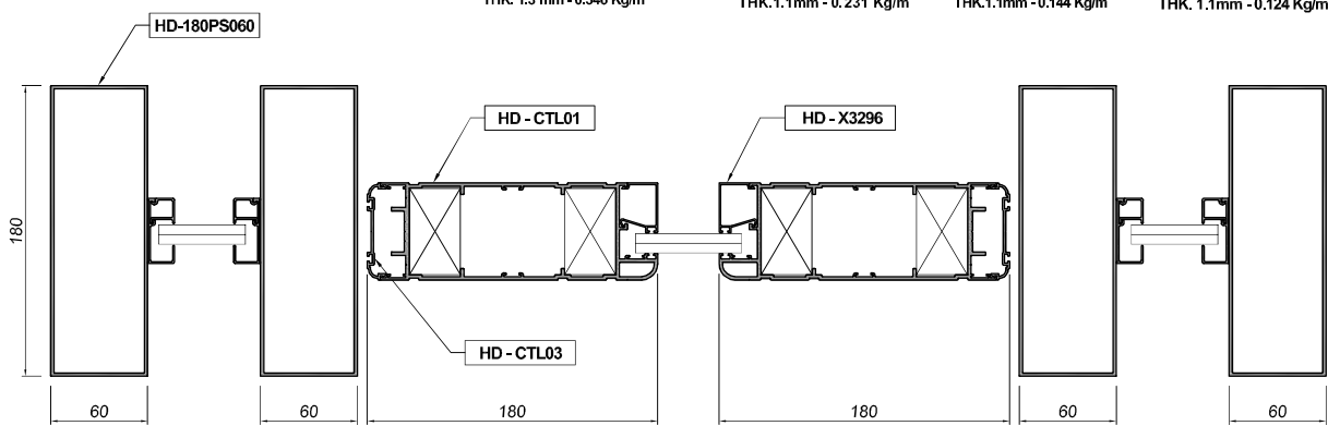
Horizontal Section Detail SCALE : NONE
