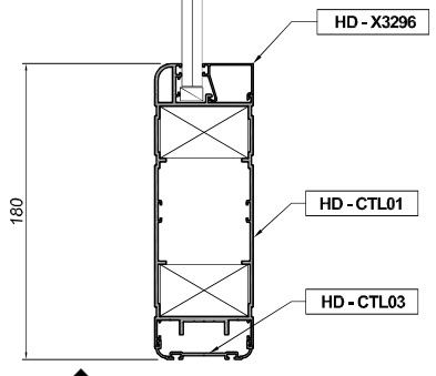
Vertical Section Detail SCALE : NONE
