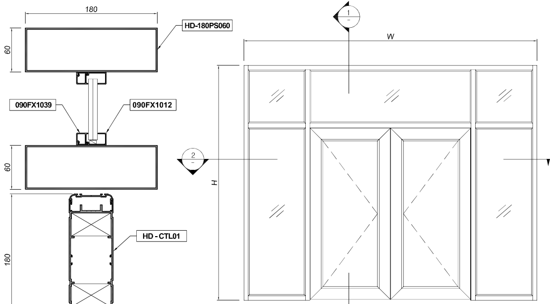
Elevation SCALE : NONE
